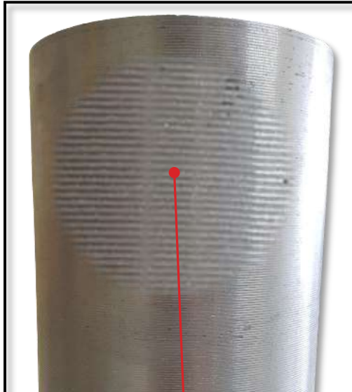
Micro Grooving on OD circumference
